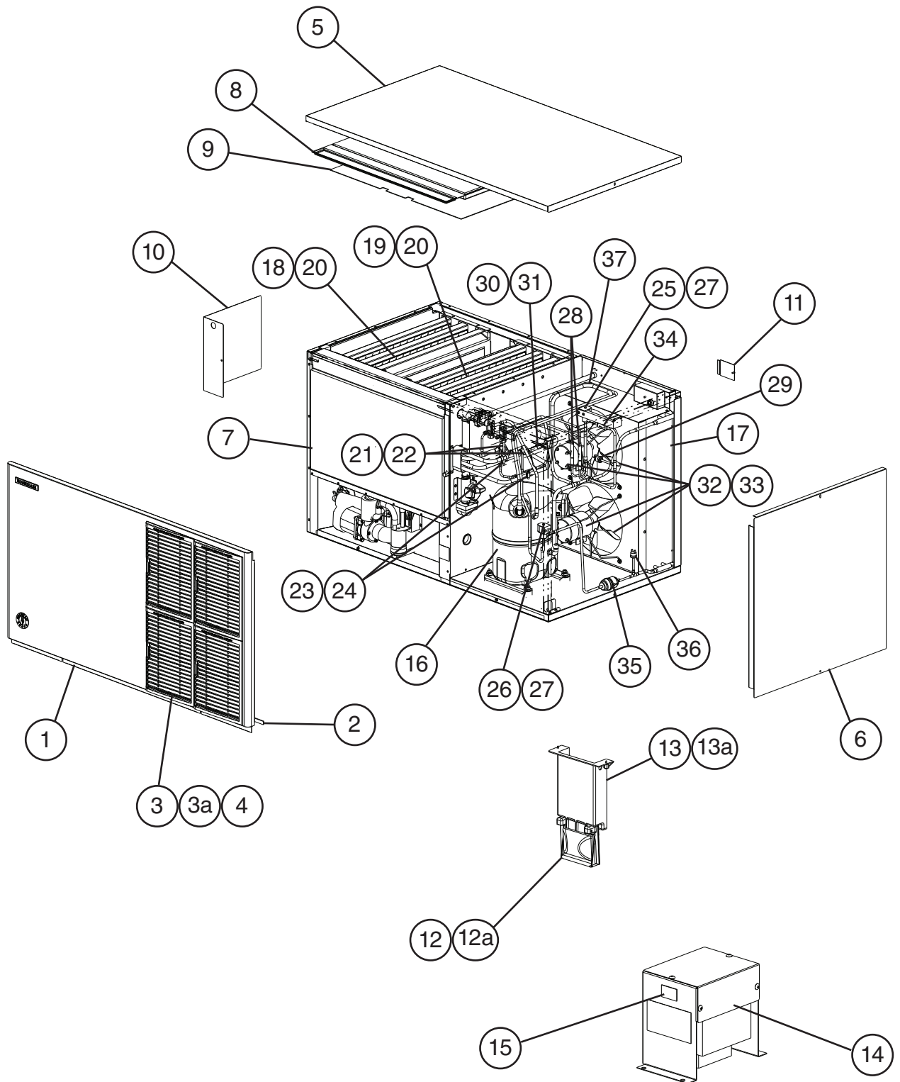
Main Transformer Box Assembly KM-1601SAJ3
